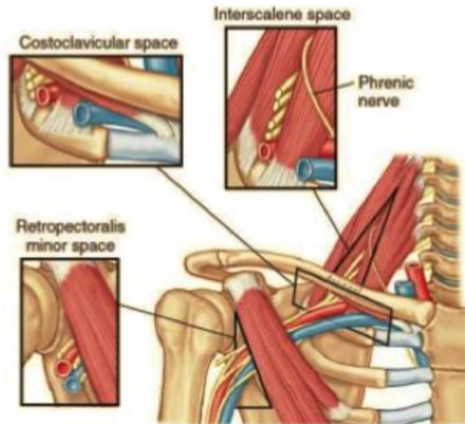
FIGURE 59-2 Three spaces in the thoracic outlet that may be responsible for thoracic outlet syndrome.
